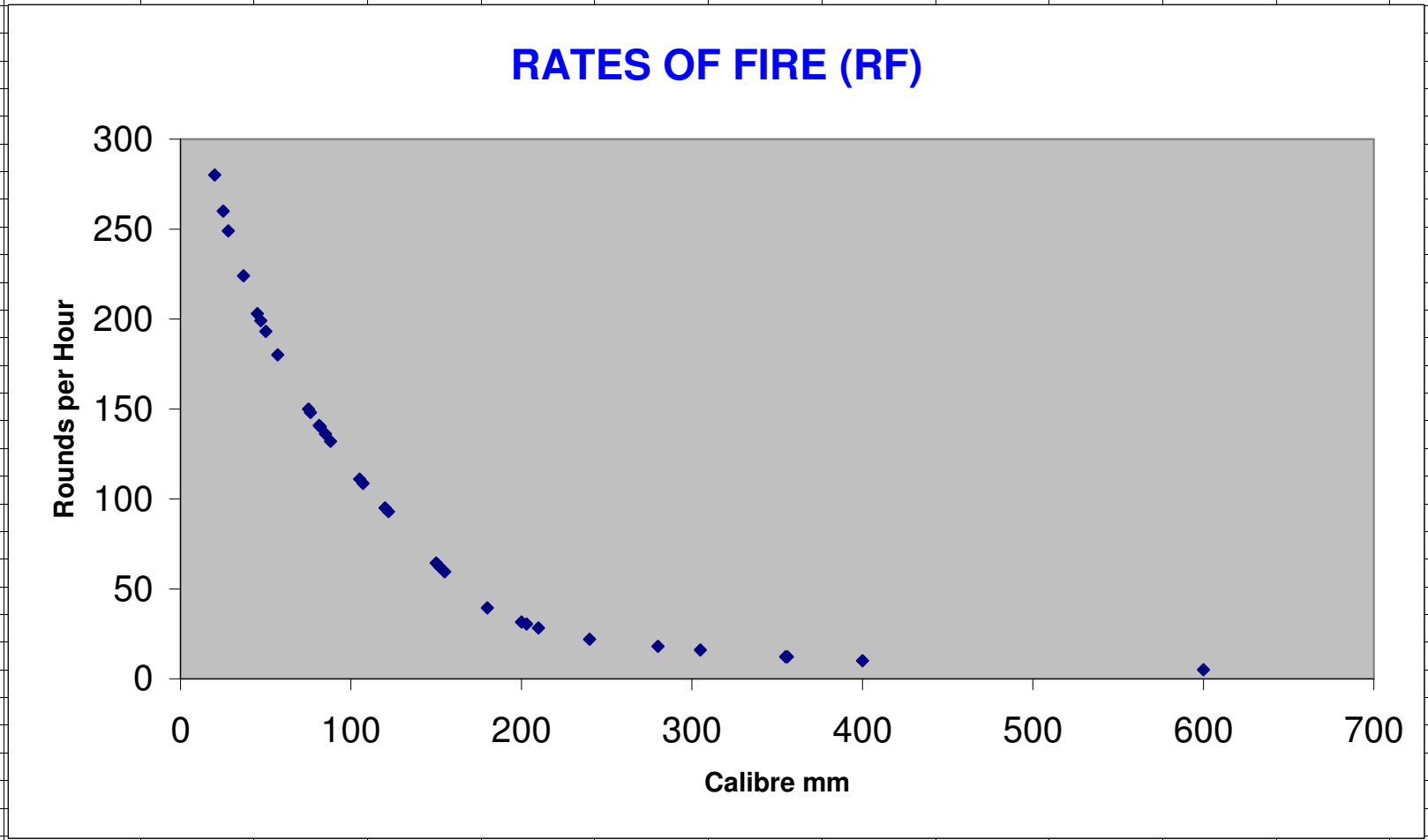
Rates of Fire vs Weapon Calibre, for non-automatic and non-AA weapons.
